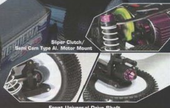
Front Universal Drive Shaft
